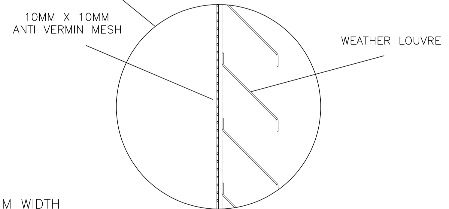
DETAIL OF INLET & OUTLET LOUVRE PANEL
