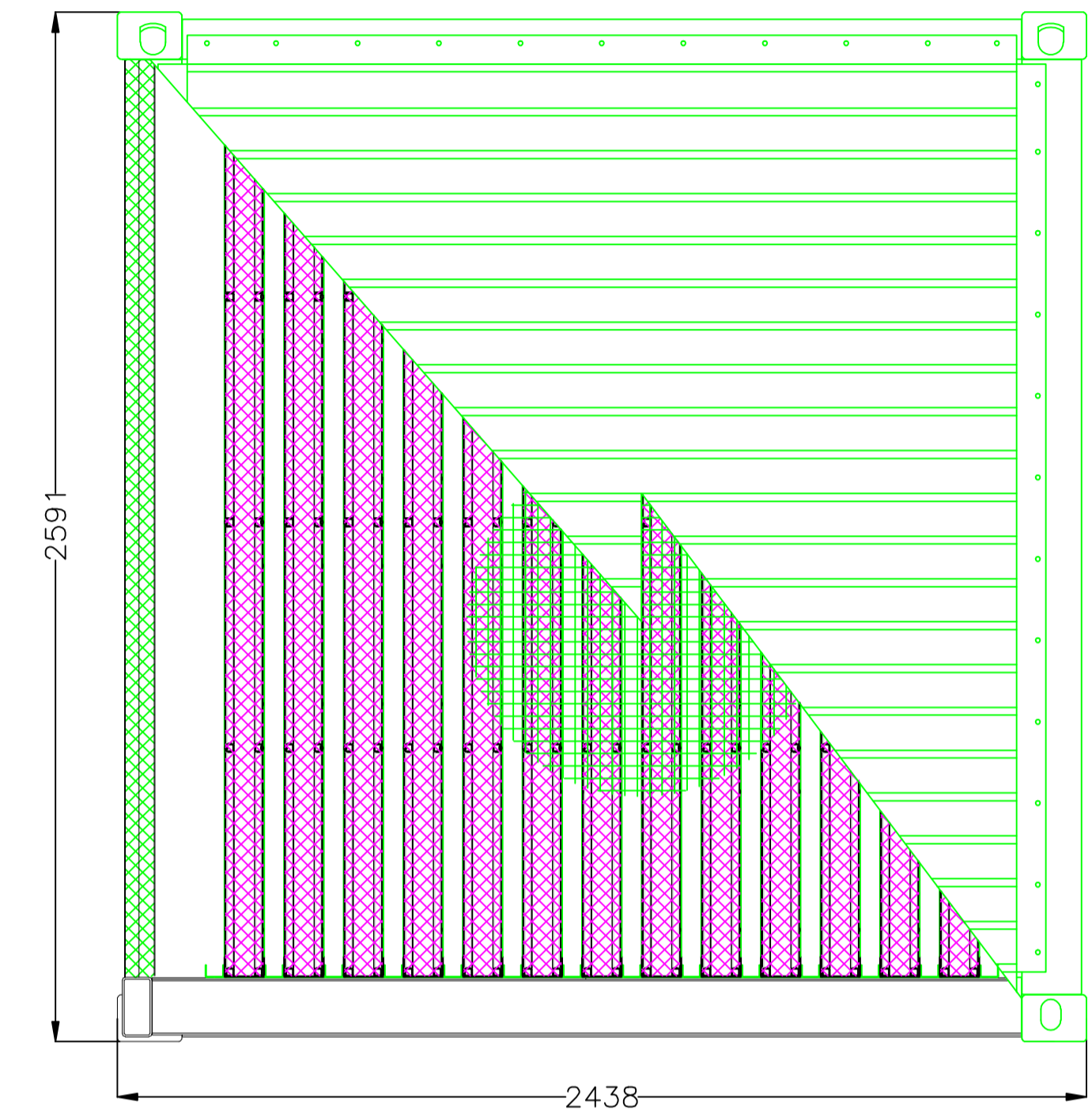
FRONT & REAR END VIEW
