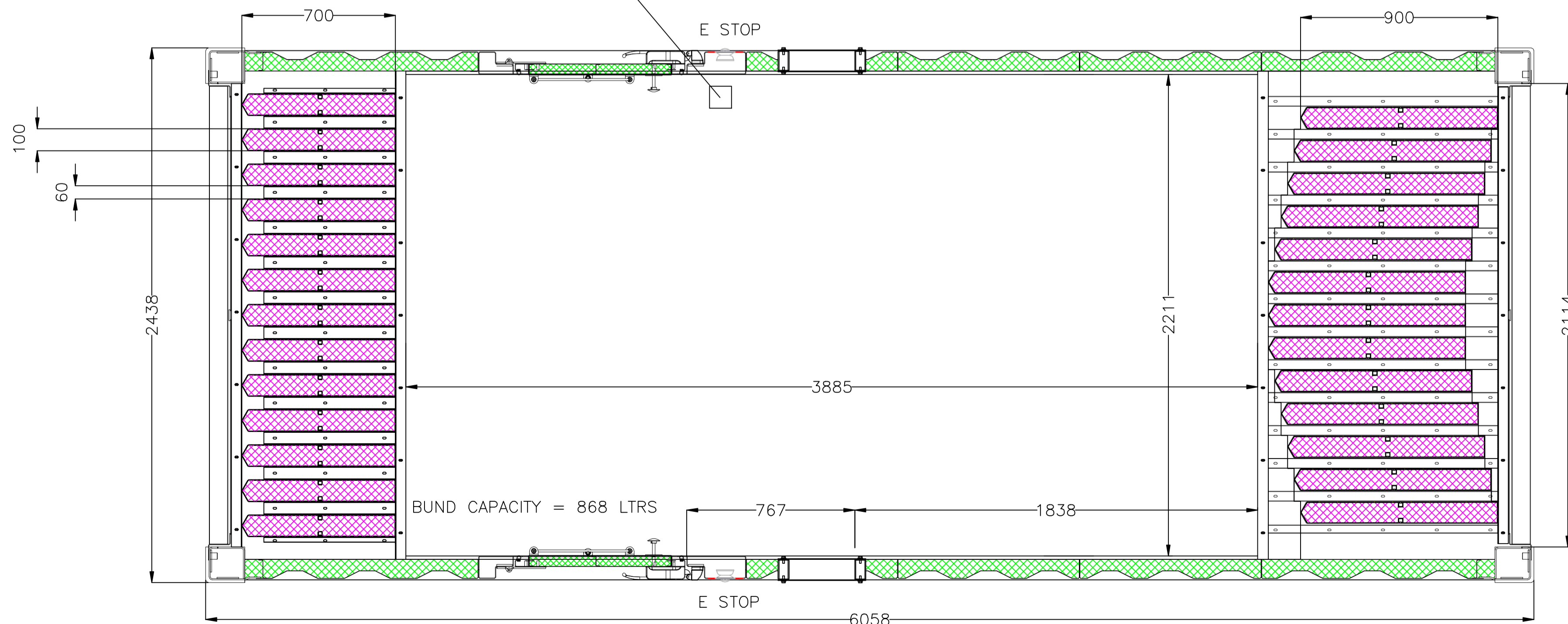
PLAN VIEW (ROOF DETAIL REMOVED)
