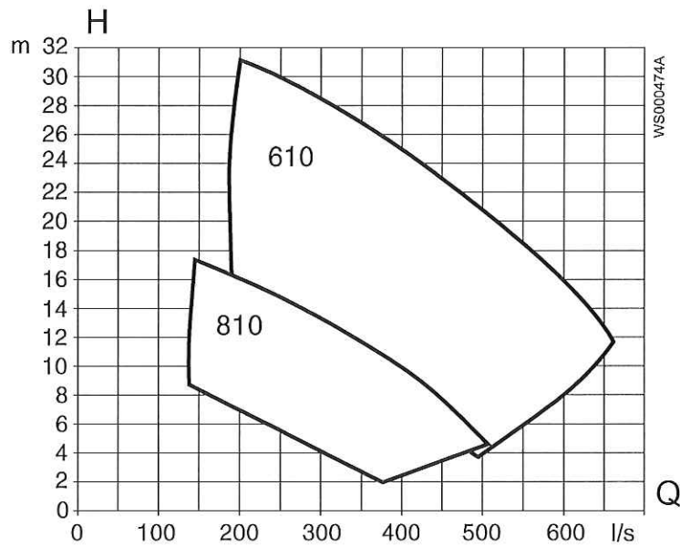
Figure 59: C3356, 50 Hz, low voltage
